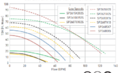
SUPER PUMP FLOW VS. TOTAL HEAD
